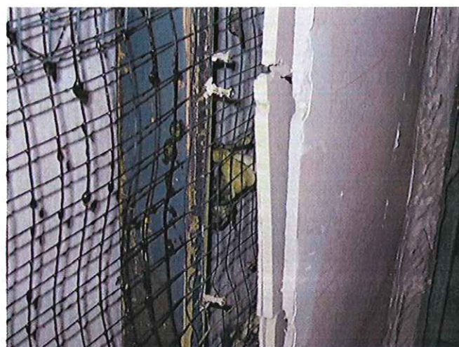
Figure C-2 (continued): The specimen after testing
